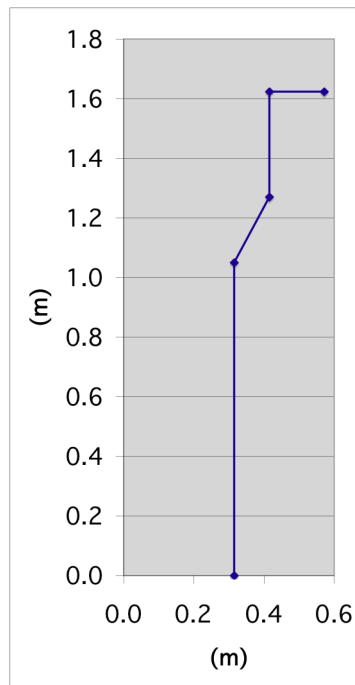
Figure 3.1-1 - Line Segments Defining Plasma Facing Surfaces
