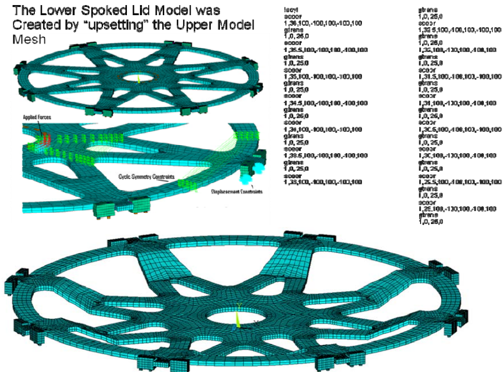
Figure 6.0-2 Symmetry Expansion of the Bent Spoke Model. and method of developing the lower spoke Model from the upper Spoked Lid Model.
