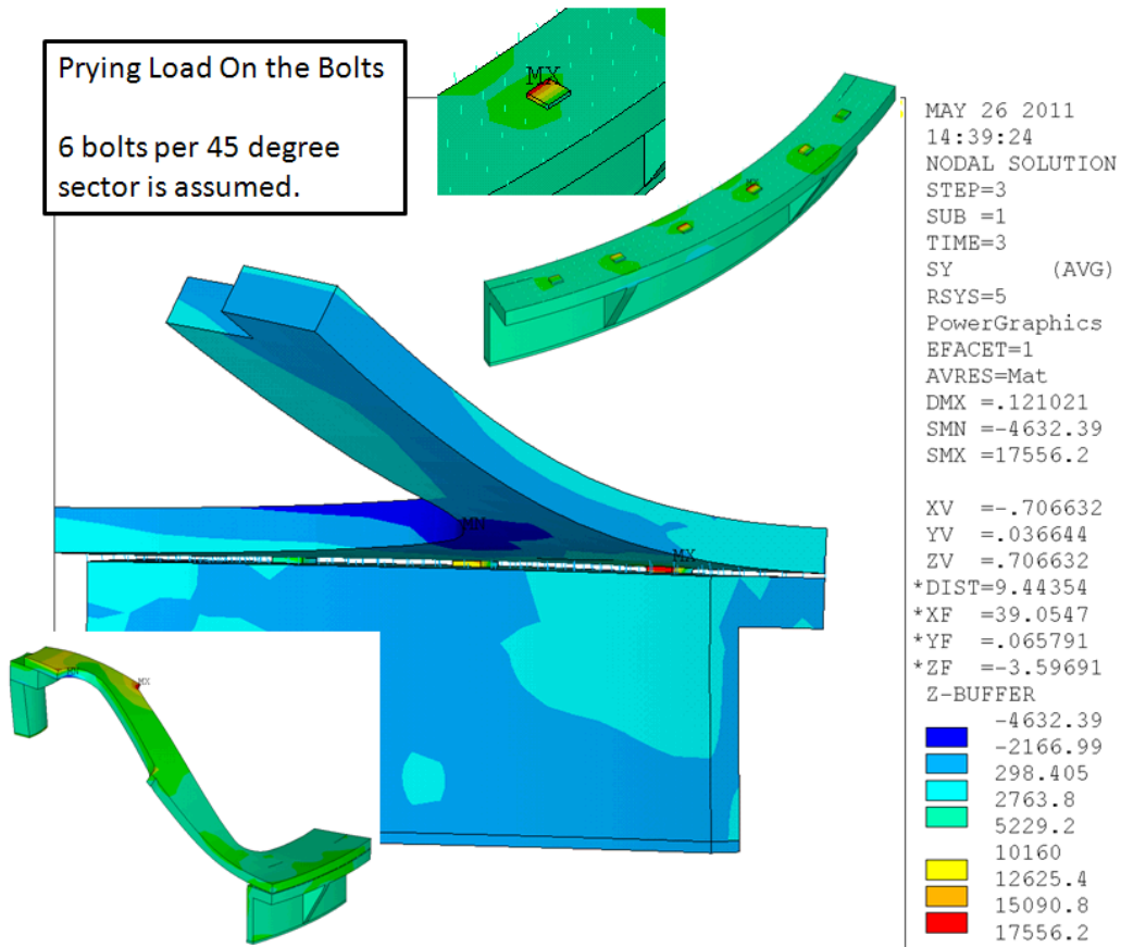
Figure 5.1-2 Spoked Lid with Bolted Outer Flange
