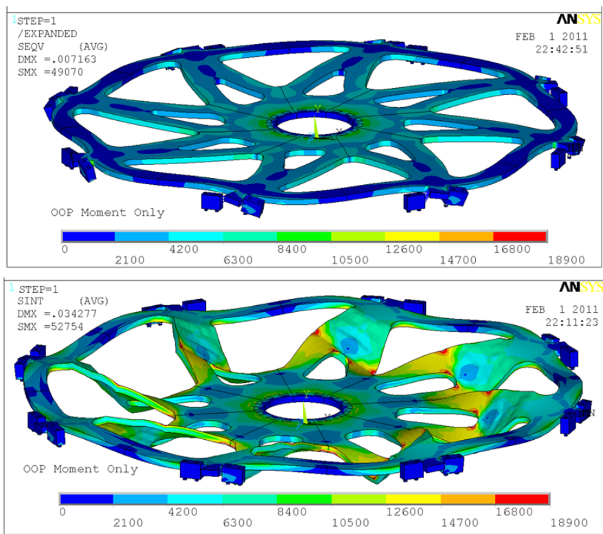
Figure 6.0-3 Results showing the Rotations of the legs Caused by the Bends
