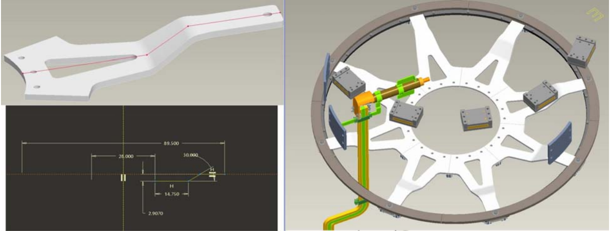
Figure 6.0-1 ProE plots of the lower spoked lid . Dimensions of the offset and View showing the routing of the OH coax lead - one of many connections passing through the lower lid.
