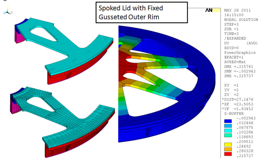
Figure 5.0-1 FDR Design Upper Lid Model
