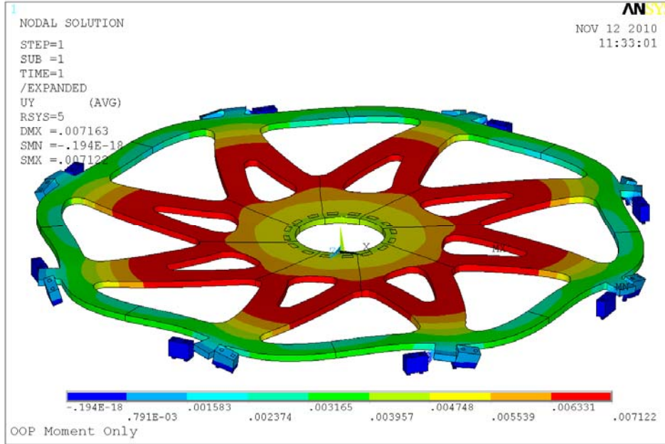
Figure 5.0-2 Pinned Outer Lug Model
