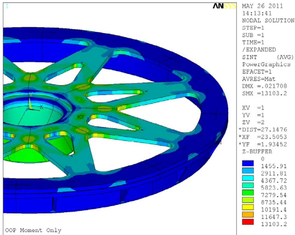
Figure 5.1-5 Spoked Lid with Bolted Outer Flange, Stress with OOP Torque Only
