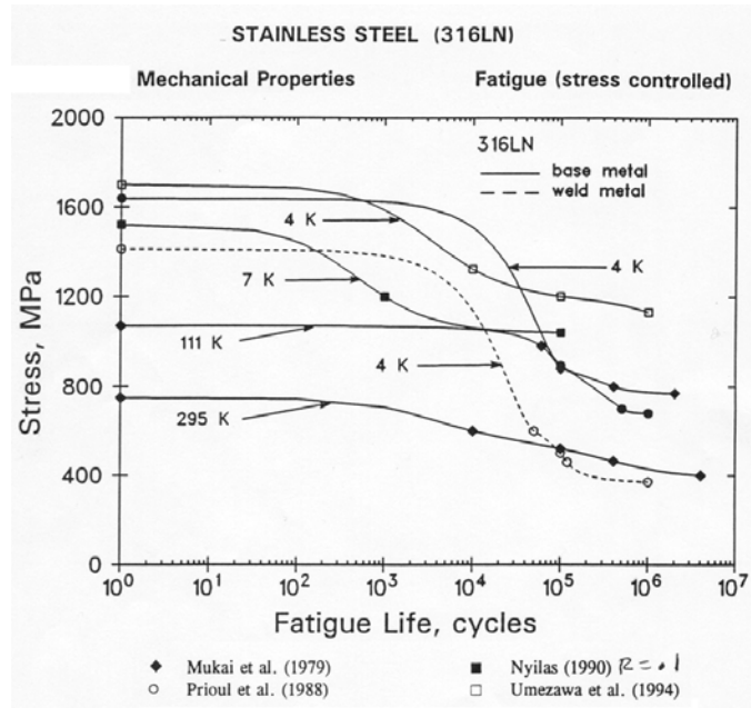
Figure 7.0-3 Fatigue S-N Curve for 316 Stainless Steel
