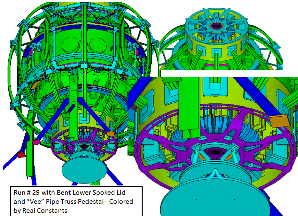
Figure 4.0-3 Global Model of the Tokamak showing the Upper and Lower Spoked Lids. In this model, the Lower "Bent" lid is shown.
