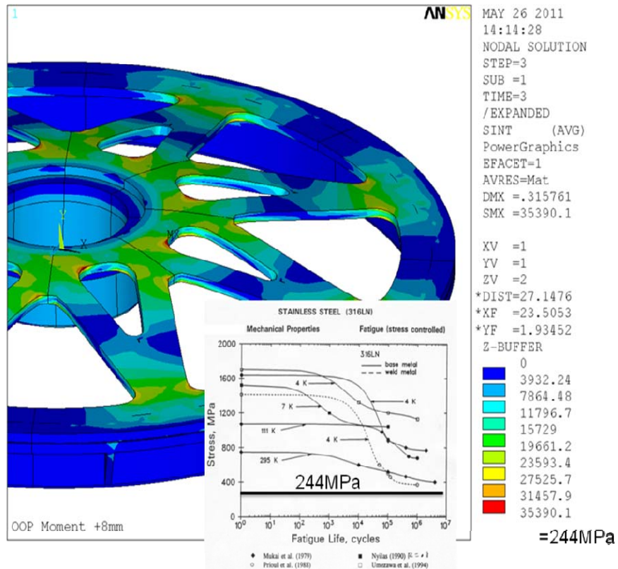
Figure 5.1-5 Spoked Lid with Bolted Outer Flange, Stress with OOP Torque Only
