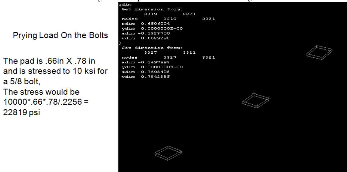
Figure 5.1-3 Spoked Lid with Bolted Outer Flange
